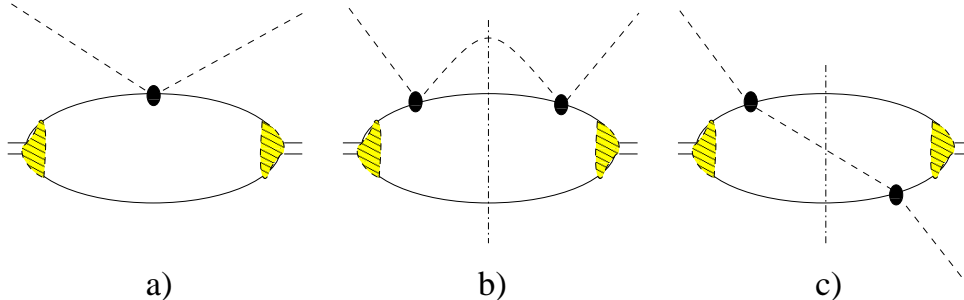
Fig. 1. Typical Feynman diagrams for \pi d scattering; shown are one-body terms (diagram a) and b), as well as the corresponding rescattering contribution c). Solid black dots stand for the \pi N interaction, whereas the hatched area shows the deuteron wave function. Crossed terms (where the external pion lines are interchanged) are not shown explicitly.
